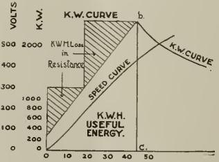
FIG. 5—ENERGY LOSSES SERIES PARALLEL CONTROL
